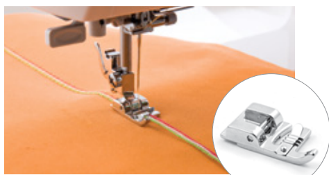
TEXI 1012 MATIC cording foot for sewing-on decorative cords or elastic strings
